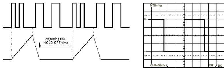
Figure 5-11(b)
