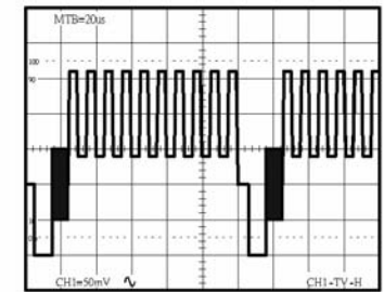
Figure 5-12(b) TV-H
