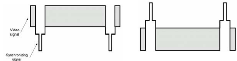
Figure 5-13(a) (┐┐) Sync signal. Figure 5-13(b) (┌┌) Sync signal
