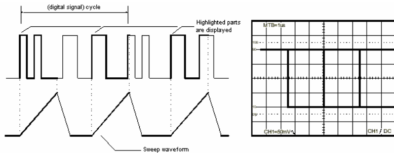
Figure 5-11(a)
