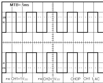
Figure 5-3 Display 1
